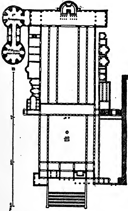
Plan of S. Peter in the Middle Ages.
